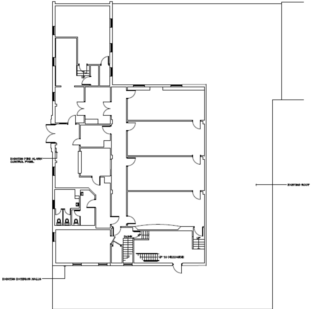
FLOOR PLAN: UPPER LEVEL: EXISTING CONDITIONS
